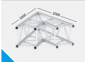
M29S-C201 129001 45° 8.72 kg
