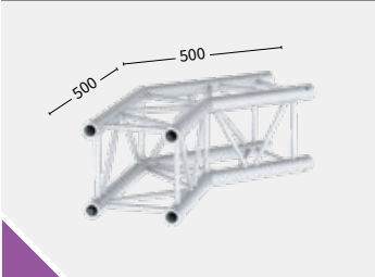
M29S-C205 129005 135° 6.21 kg
