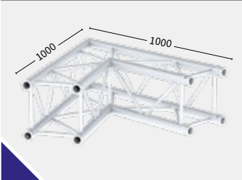
M29S-C202 129002 60° 9.61 kg
